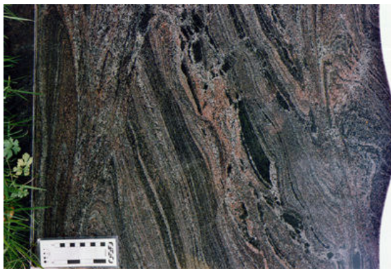
Gneiss
