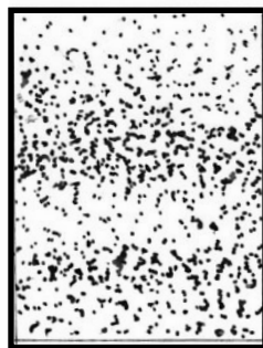
Diffuse modal with gradational contacts
